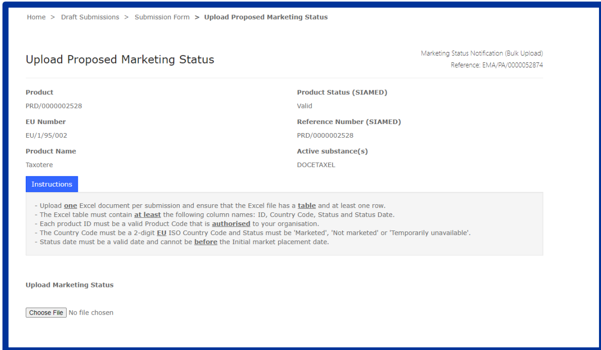
Figure 21: Upload CSV file
